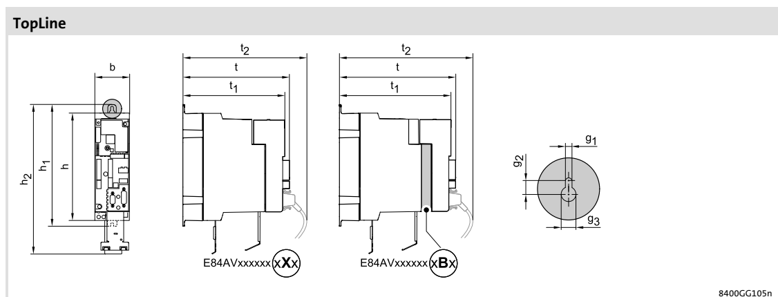
Fig. 5-3 Device dimensions
