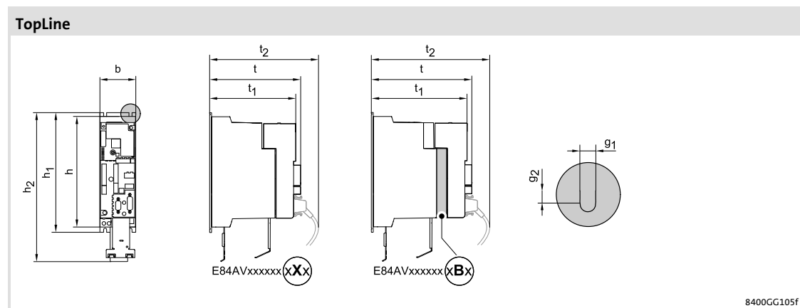
Fig. 5-17 Device dimensions
