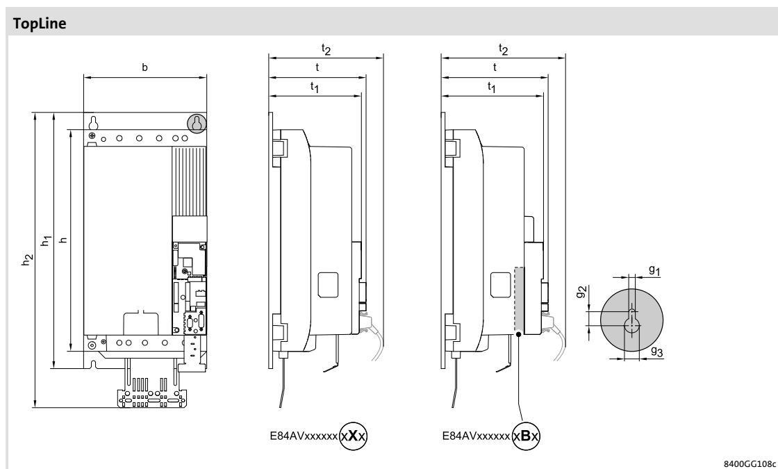
Fig. 5-47 Device dimensions
