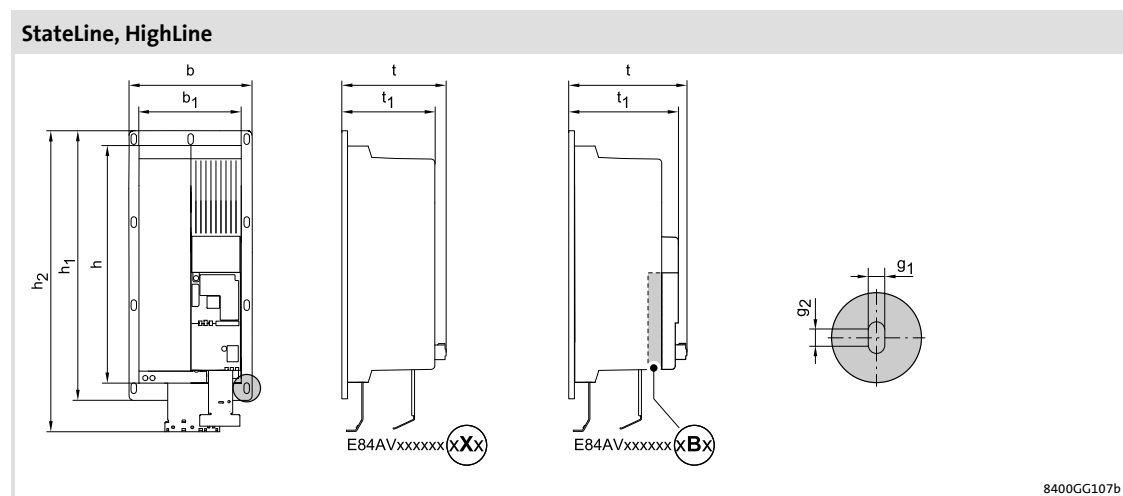
Fig. 5-37 Device dimensions
