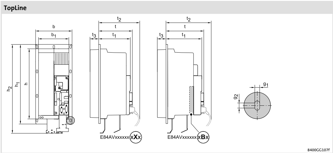
Fig. 5-31 Device dimensions
